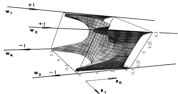
Fig. 4 3D-plot of RF field generated by two long parallel coils placed into the horizontally oriented stationary magnetic field \mathbf{B}_0 .
