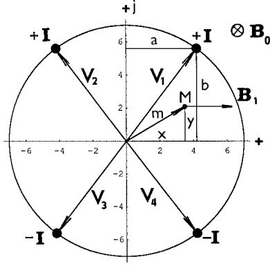
Fig.1 Four conductors placed on a cylinder supplied by currents +I and -I are generating the RF field in the central region. The field \mathbf{B}_1 in the point M is calculated.
