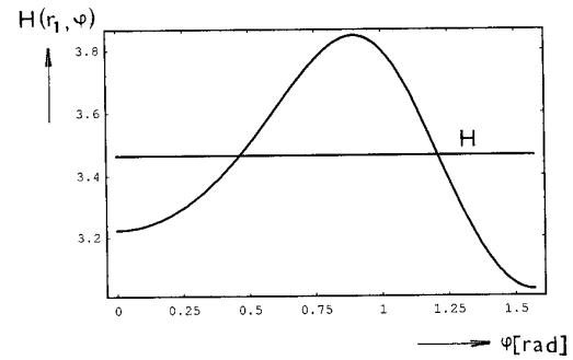
Fig. 3 A plot of the field on the circular line and the field in the origin in rectangular coordinates
