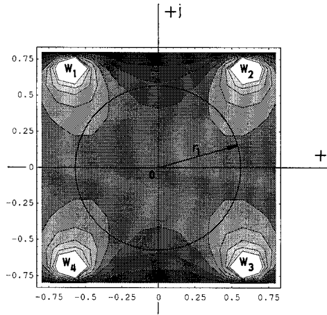
Fig. 2 The relative contour plot of the optimised RF field generated by four conductors. The evaluated circular line has the relative radius r_1 = 0.6 .
